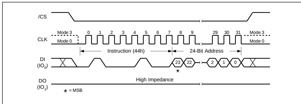
Figure 45. Erase Security Registers Instruction Sequence(SPI mode only)
